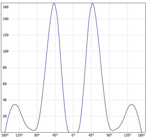
Luminance Distribution
